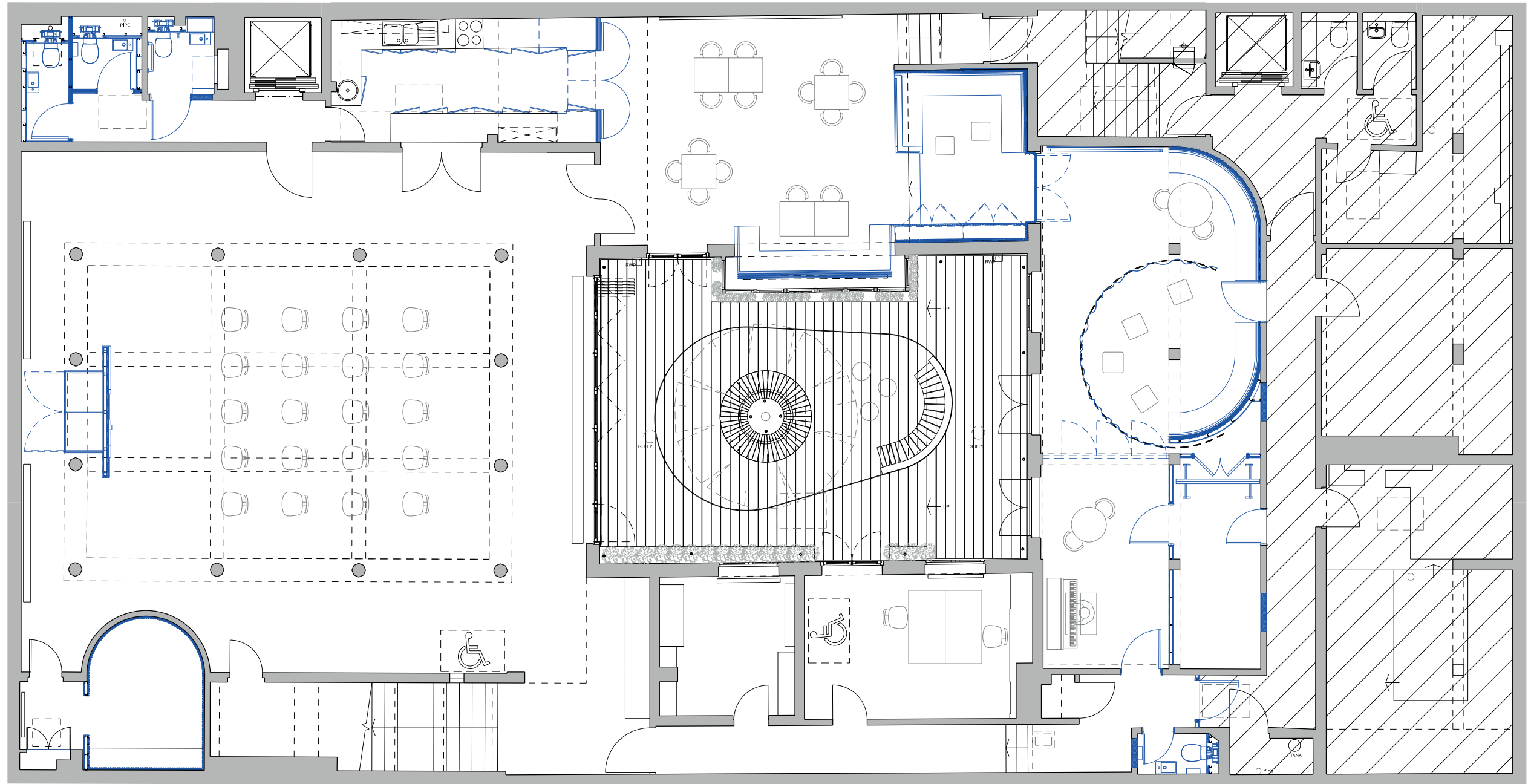
Basement Floor Plan 1:100 @ A3
